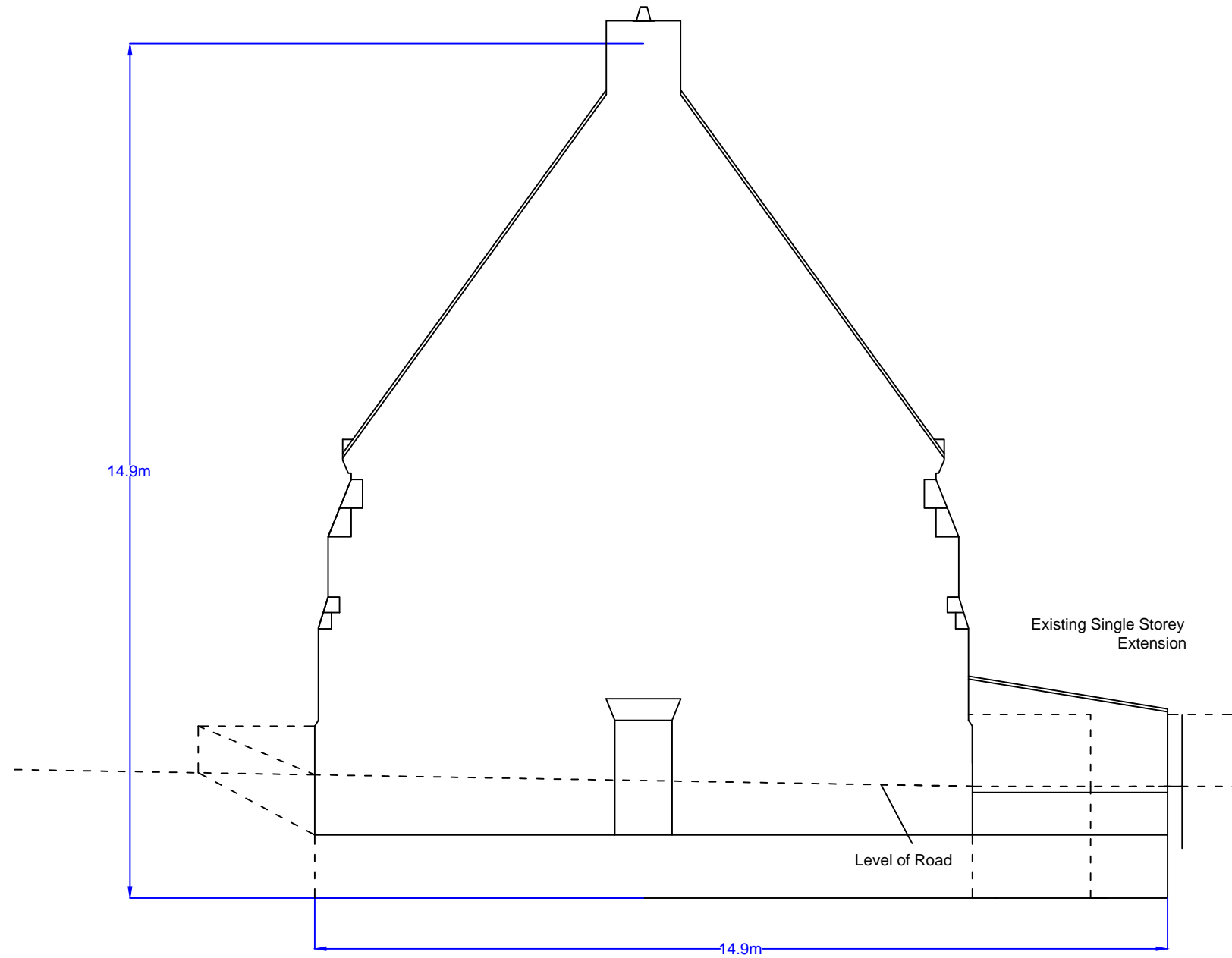
8DT10: 8 Derby Terrace South Elevation As Proposed Page 1 of 1, Scale 1:100 at A3
